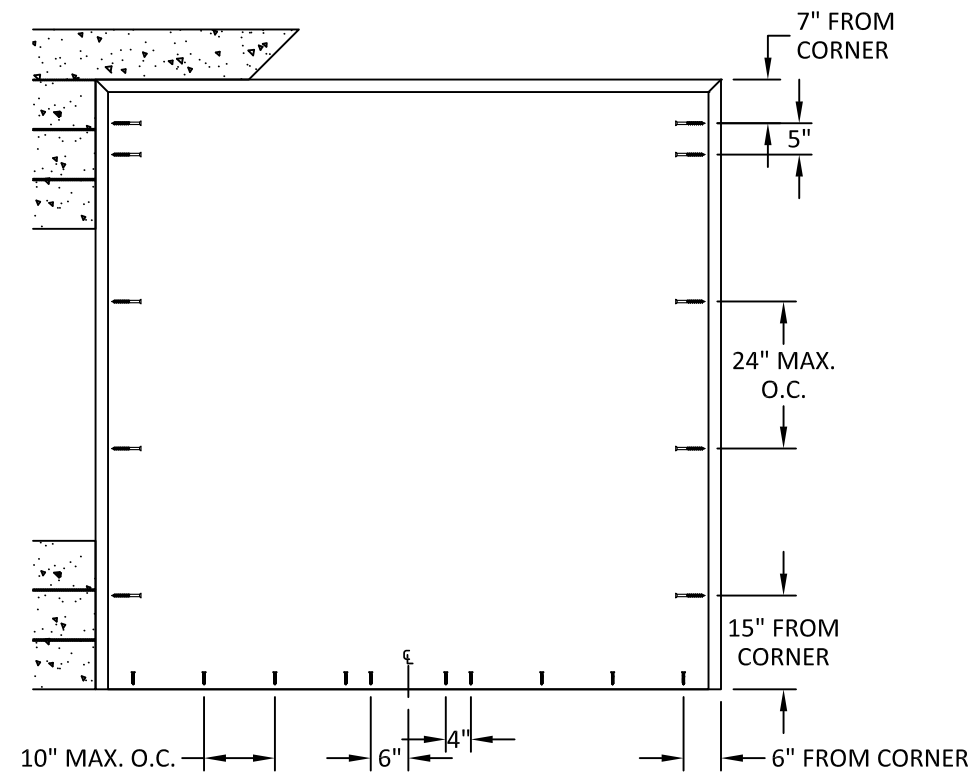
ANCHOR LAYOUT CONCRETE SUBSTRATE TUBE/BUTTERFLY ANCHOR ELEVATION # 4, 5, & 6
