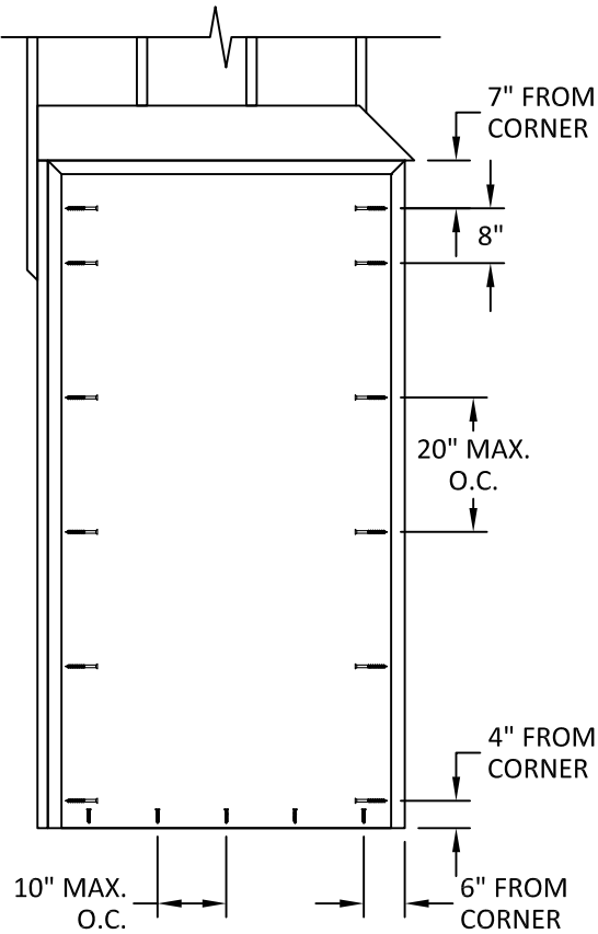
ANCHOR LAYOUT WOOD/METAL STUDS TUBE/BUTTERFLY ANCHOR ELEVATION # 1, 2, & 3
