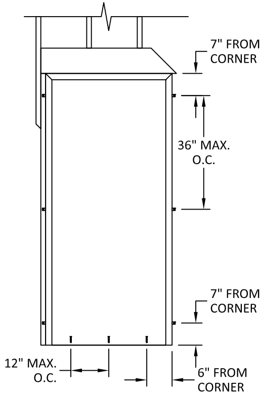
ANCHOR LAYOUT WOOD/METAL STUDS STUD STRAP ANCHOR ELEVATION # 7, 8, 9, & 10
