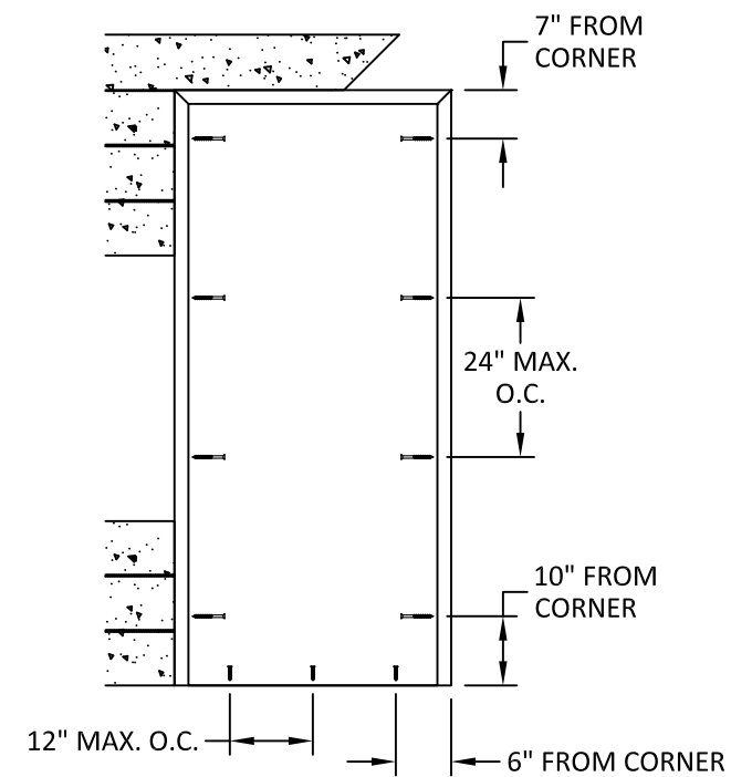
ANCHOR LAYOUT CONCRETE SUBSTRATE TUBE/BUTTERFLY ANCHOR ELEVATION # 7, 8, 9, & 10
