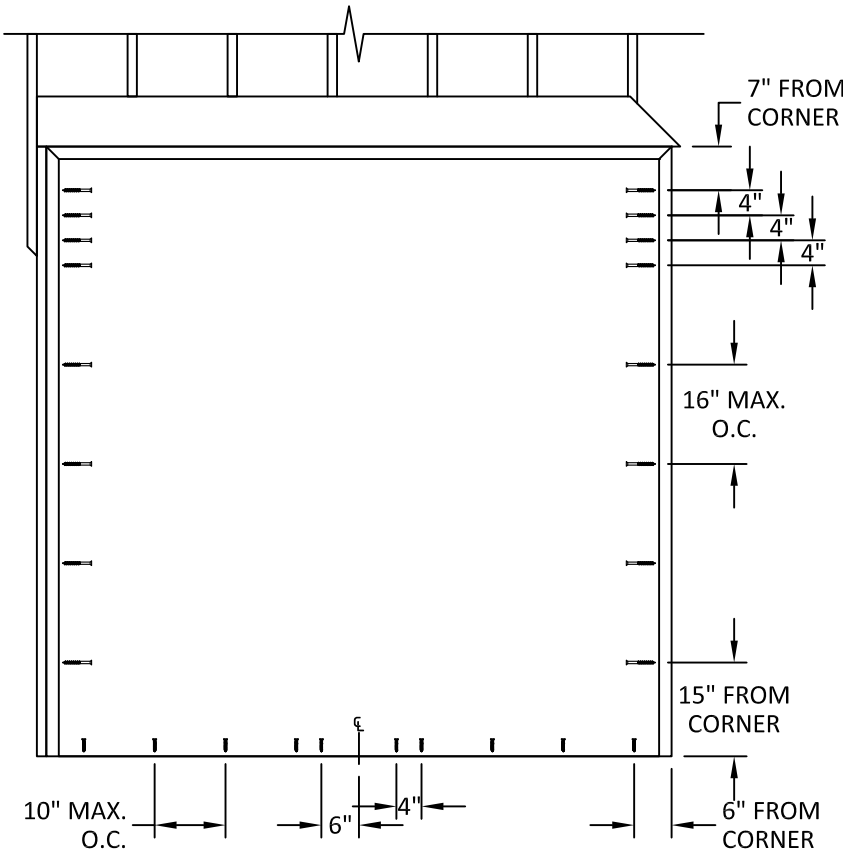
ANCHOR LAYOUT WOOD/METAL STUDS TUBE/BUTTERFLY ANCHOR ELEVATION # 4, 5, & 6
