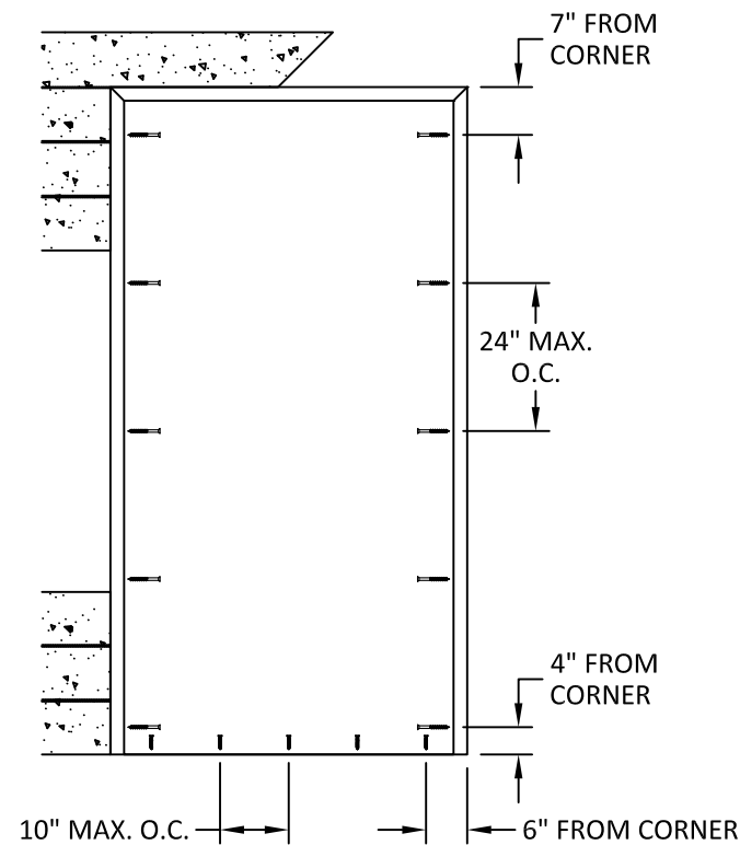
ANCHOR LAYOUT CONCRETE SUBSTRATE TUBE/BUTTERFLY ANCHOR ELEVATION # 1, 2, & 3
