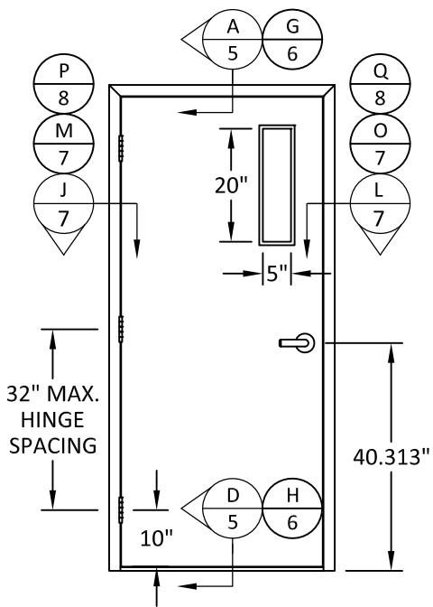
ELEVATION #9 INSWING/OUTSWING SINGLE DOOR
