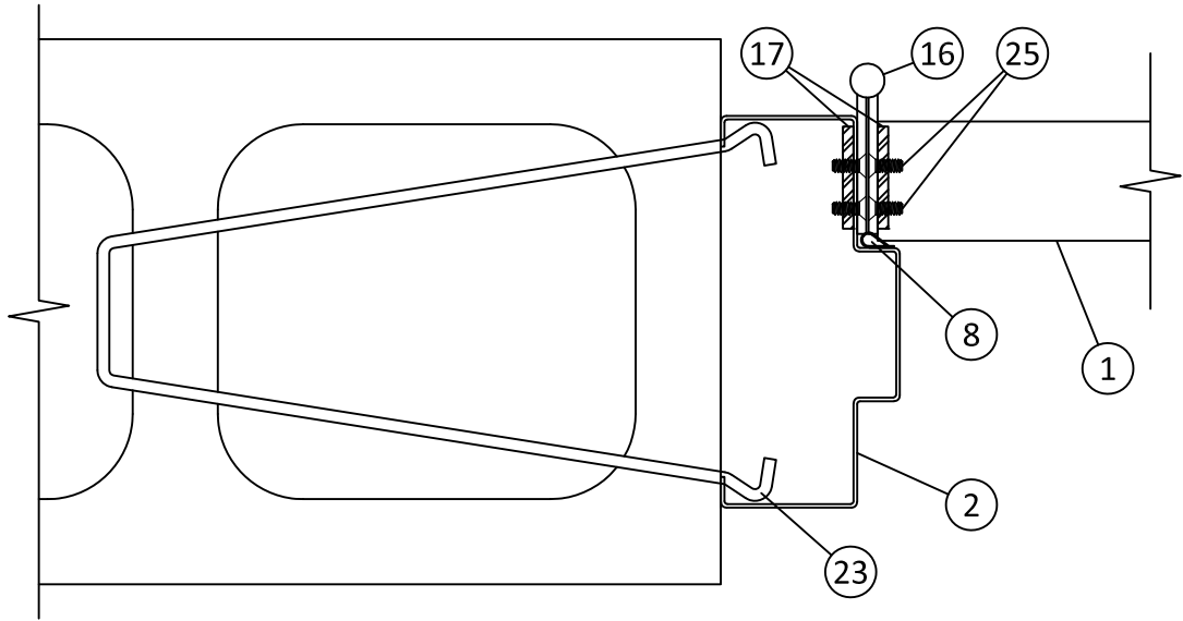
P 8 HORIZONTAL SECTION IN SWING DOOR HINGE JAMB
