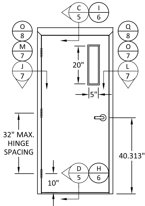
ELEVATION #10 INSWING/OUTSWING SINGLE DOOR W/ 4" HEADER
