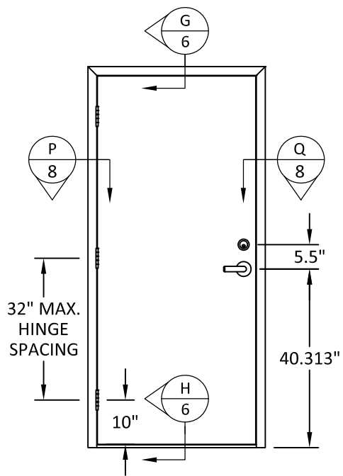
ELEVATION #7 INSWING SINGLE DOOR
