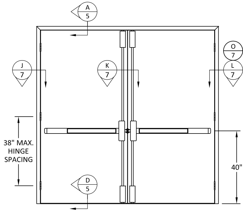
ELEVATION #6 OUTSWING DOUBLE DOOR
