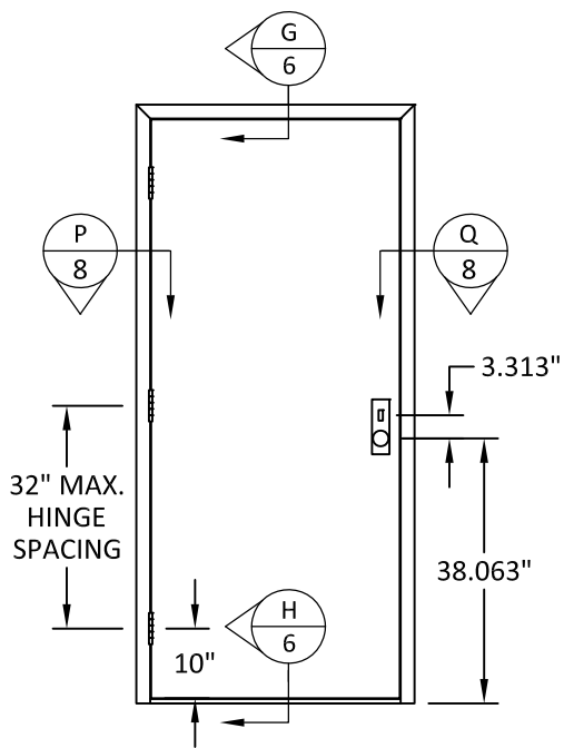
ELEVATION #8 INSWING SINGLE DOOR
