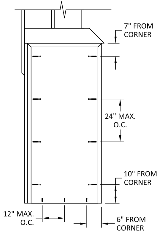
ANCHOR LAYOUT WOOD/METAL STUDS TUBE/BUTTERFLY ANCHOR ELEVATION # 7, 8, 9, & 10
