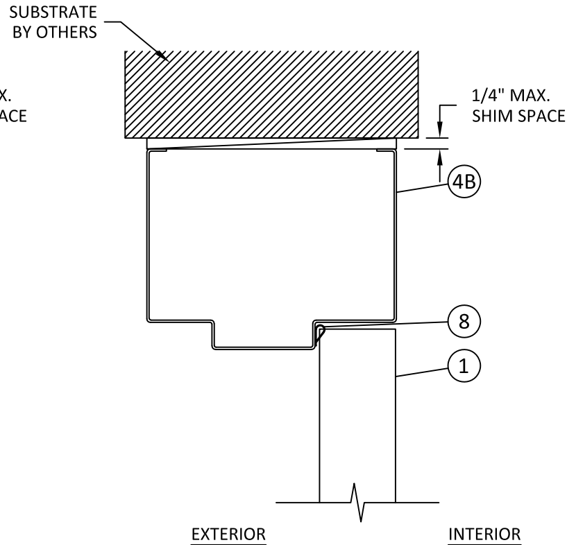
I 6 VERTICAL SECTION INSWING DOOR HEAD 4" HEADER
