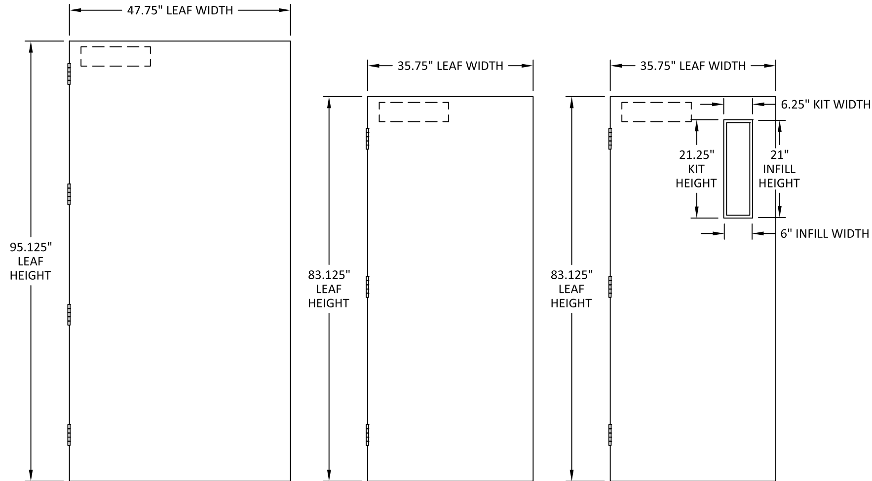
8'-0" DOOR LEAF ELEVATIONS # 1, 2, 3, 4, 5, & 6
