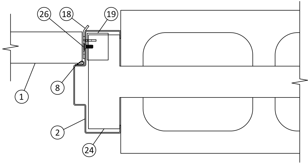
Q 8 HORIZONTAL SECTION IN SWING DOOR LOCK JAMB
