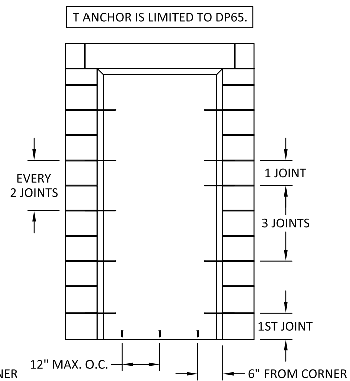
ANCHOR LAYOUT CONCRETE SUBSTRATE WIRE/T ANCHOR ELEVATION # 7, 8, 9, & 10
